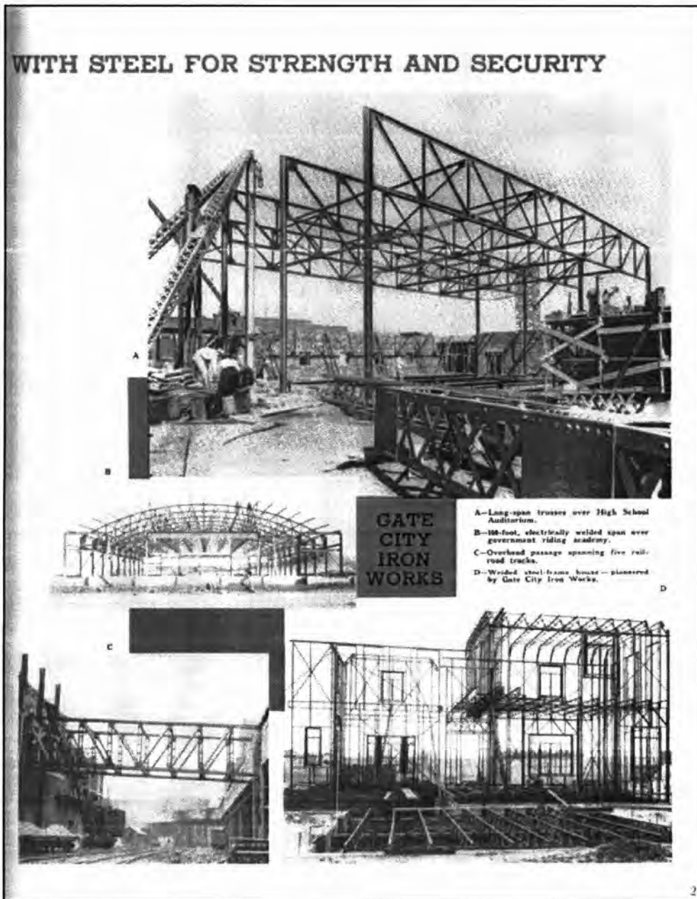
Photo 5: The catalog entry Item D (lower right) reads, "Welded steel-frame house—pioneered by Gate City Iron Works." Photo Credit, Ornamental Iron for Enduring Beauty and Strength (Omaha, Nebraska: Gate City Iron Works, undated catalog), 25.
