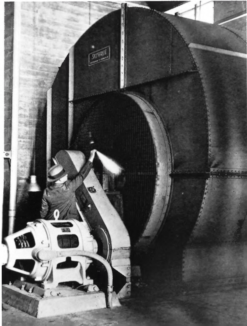
Photograph #9 Holland Tunnel New York County, NY & Hudson County, NJ Interior View of Ventilation Building, Showing An Intake Fan Gray's, The Eighth Wonder , 1927
