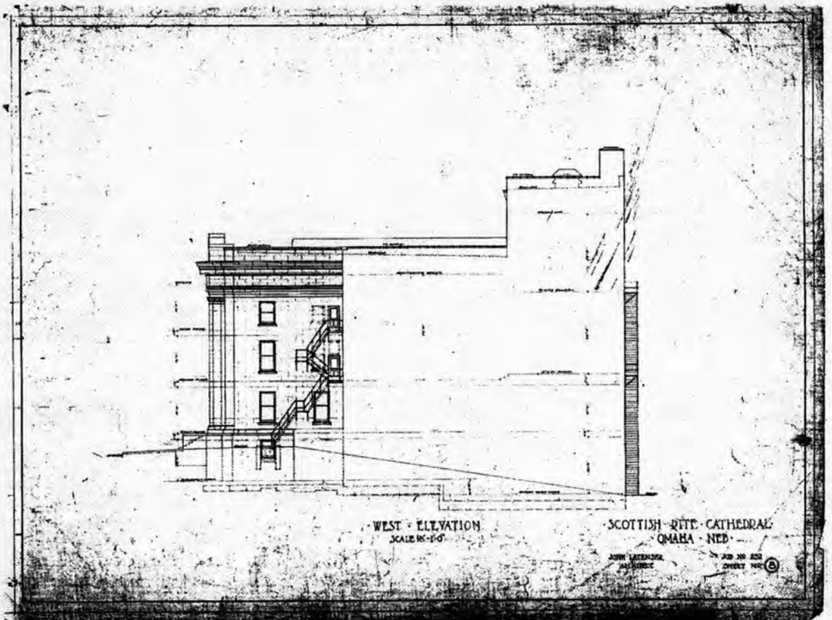
WEST ELEVATION
