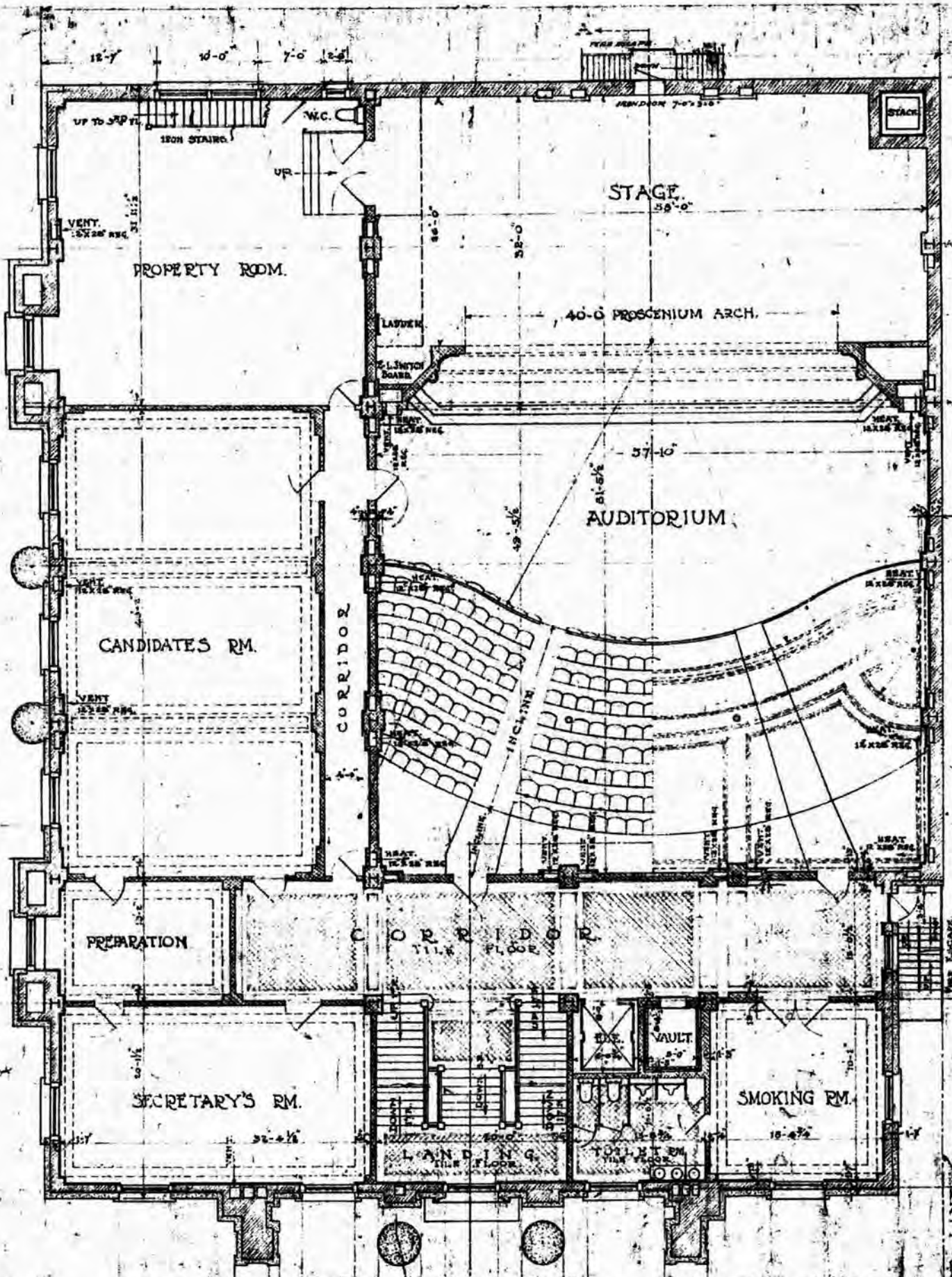
SECOND FLOOR PLAN ORIGINAL - 1912 SCOTTISH RITE CATHEDRAL
