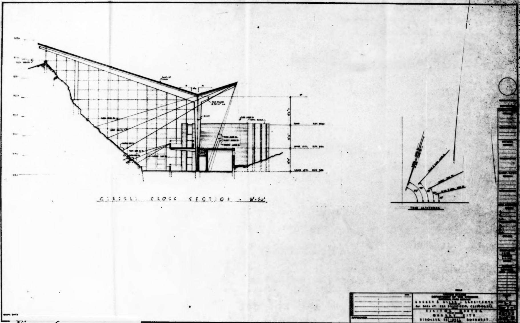
Figure 6 Quarry Visitor Center Uintah County, Utah General Cross Section
