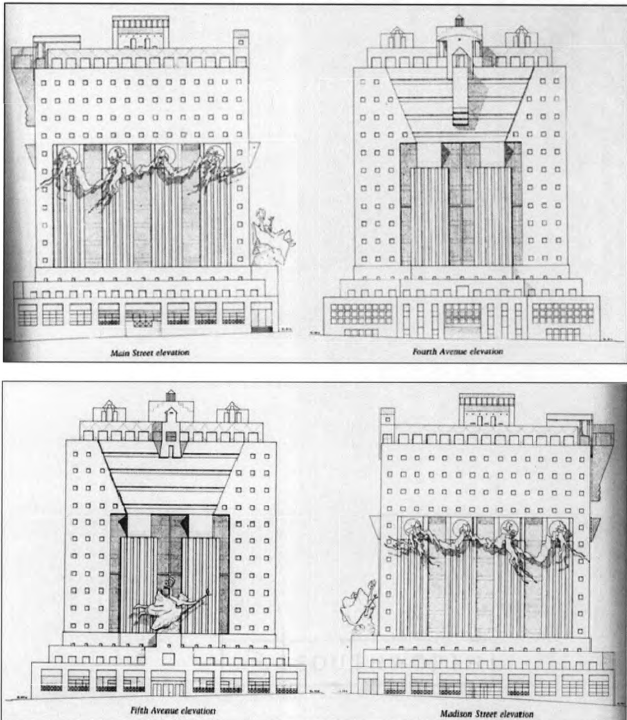
Figure 5: Building Elevations published in Michael Graves's monograph (not as constructed), c 1981
