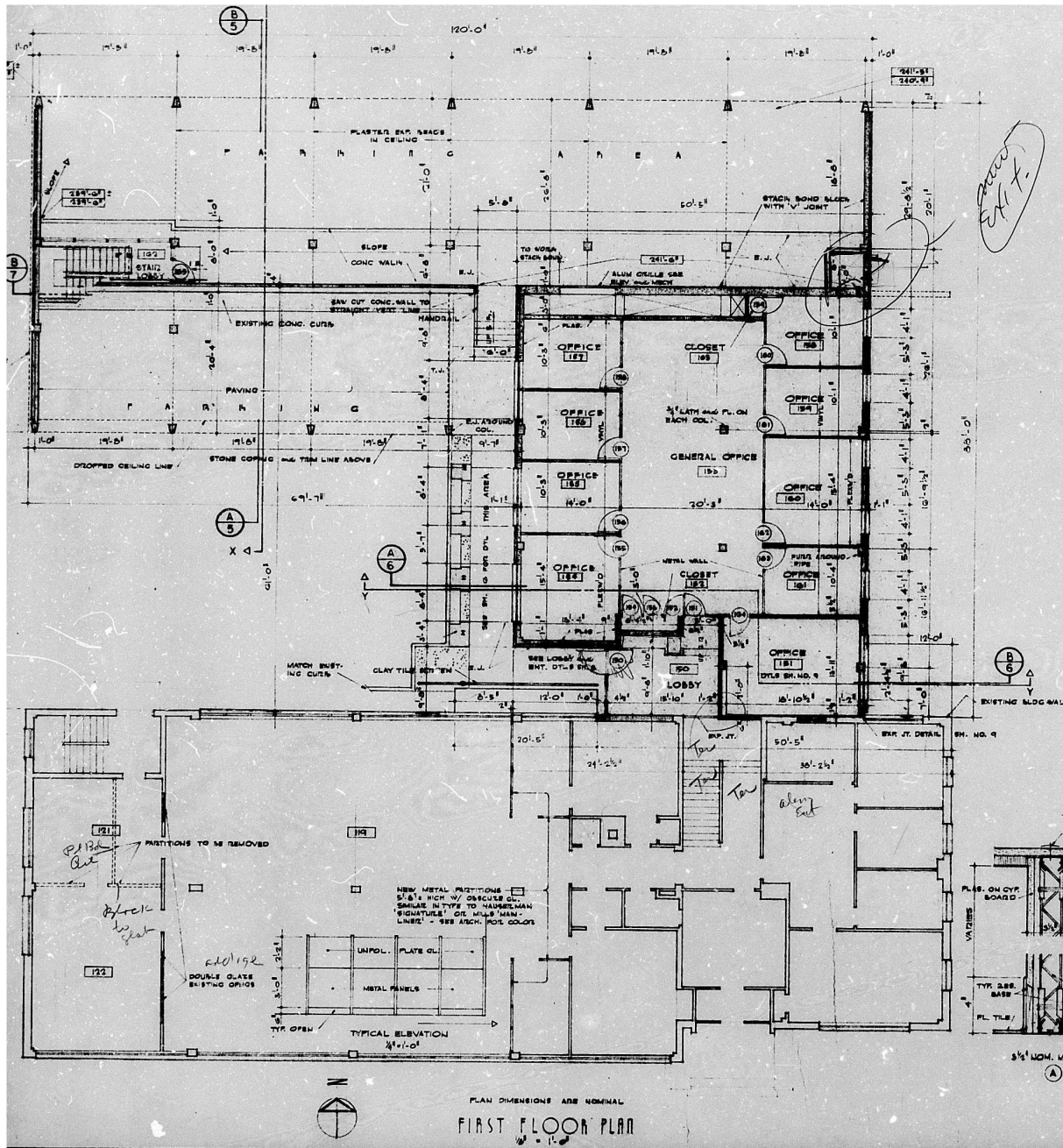
Figure 7. Historic first floor plan showing both wings, 1961. 1961 wing shown darker. Note the partitions in 1952 wing that are marked to be removed and new glazed partitions sketched in. Source: State Historical Society of Missouri, Kansas City.
