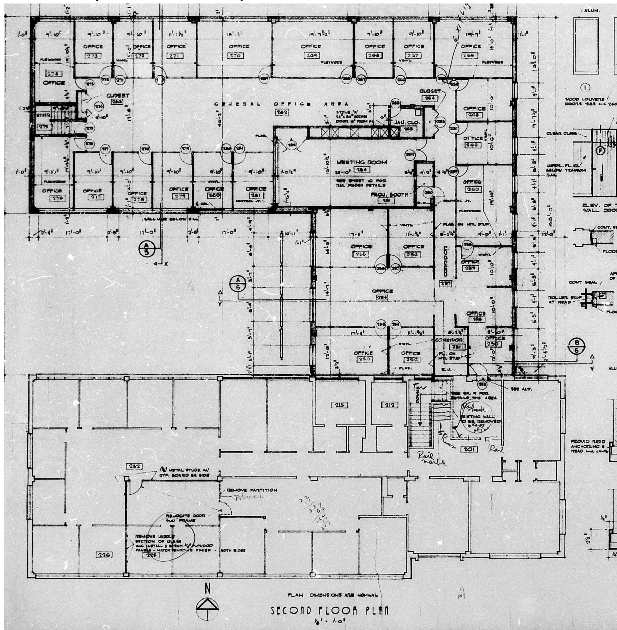
Figure 8. Historic second floor plan showing both wings. 1961 wing shown darker. Source: State Historical Society of Missouri, Kansas City.
