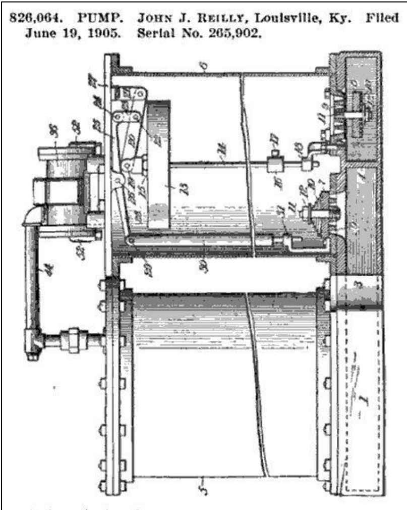
Patent for the Ideal Pump held by John J. Reilly
