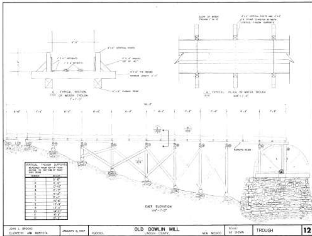
Figure 24 Architectural Drawing #8 of 9 Flume and Foundation
