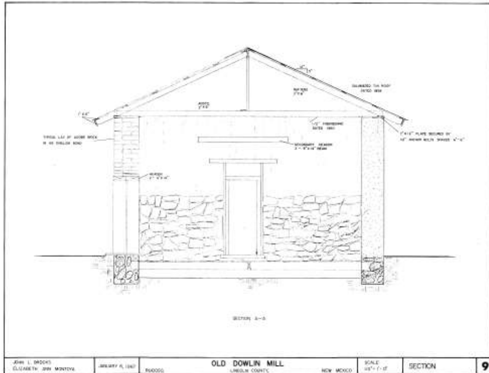
Figure 22 Architectural Drawing #6 of 9 Wall Section
