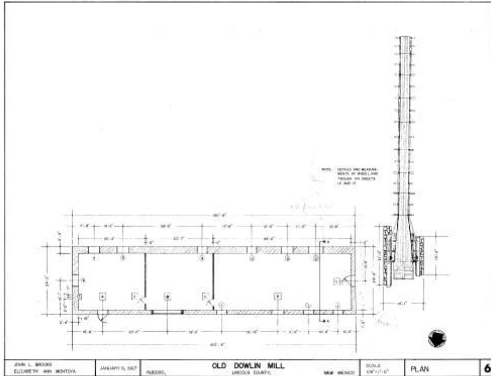
Figure 19 Architectural Drawing #3 of 9 Floor Plan
