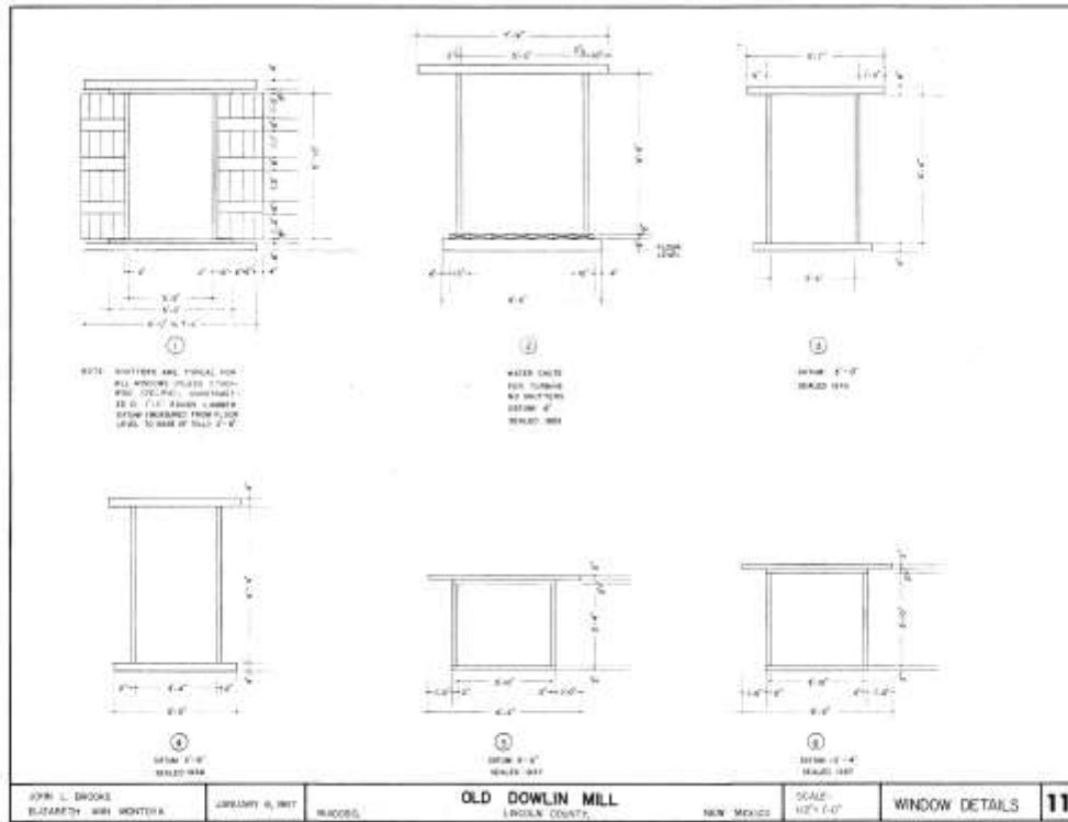
Figure 23 Architectural Drawing #7 of 9 Window Details
