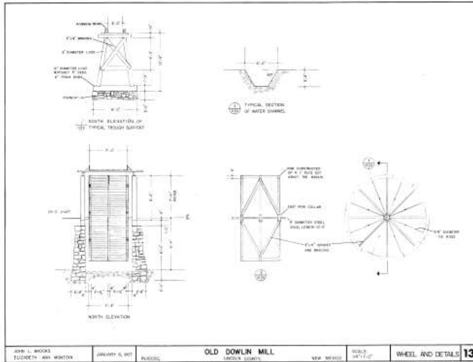
Figure 25 Architectural Drawing #9 of 9 Water-wheel and Foundation Details
