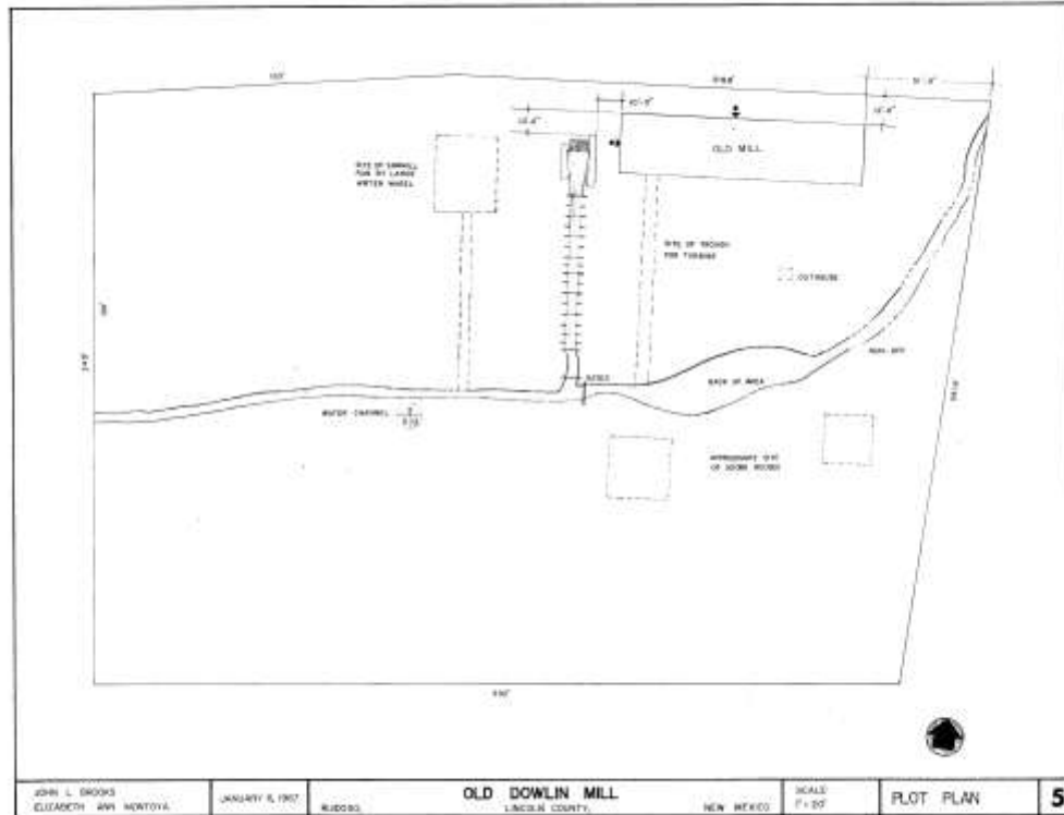
Figure 18 Architectural Drawing #2 of 9 Plot Plan
