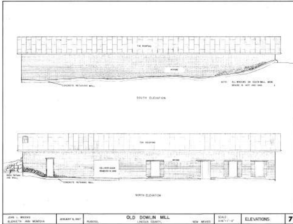
Figure 20 Architectural Drawing #4 of 9 South and North Elevation
