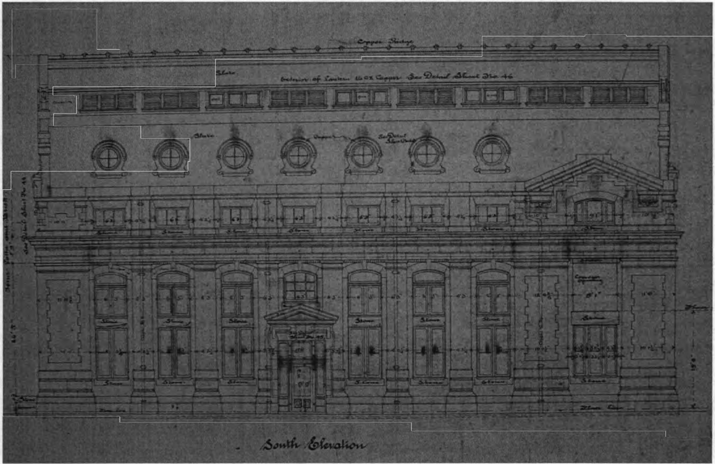
South Elevation, Sewerage Pumping Station C.A. Didden & Son, Architects and Oscar Vogt, Associate Architect, ca. 1902 Department of General Services, Archives (Reeves Center, B-2)
