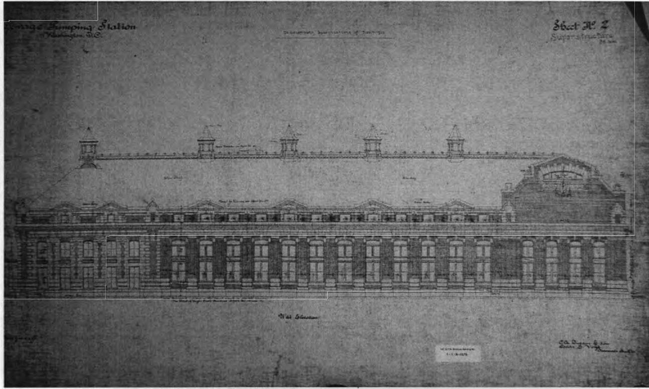
West Elevation, Sewerage Pumping Station C.A. Didden & Son, Architects and Oscar Vogt, Associate Architect, ca. 1902 Department of General Services, Archives (Reeves Center, B-2)
