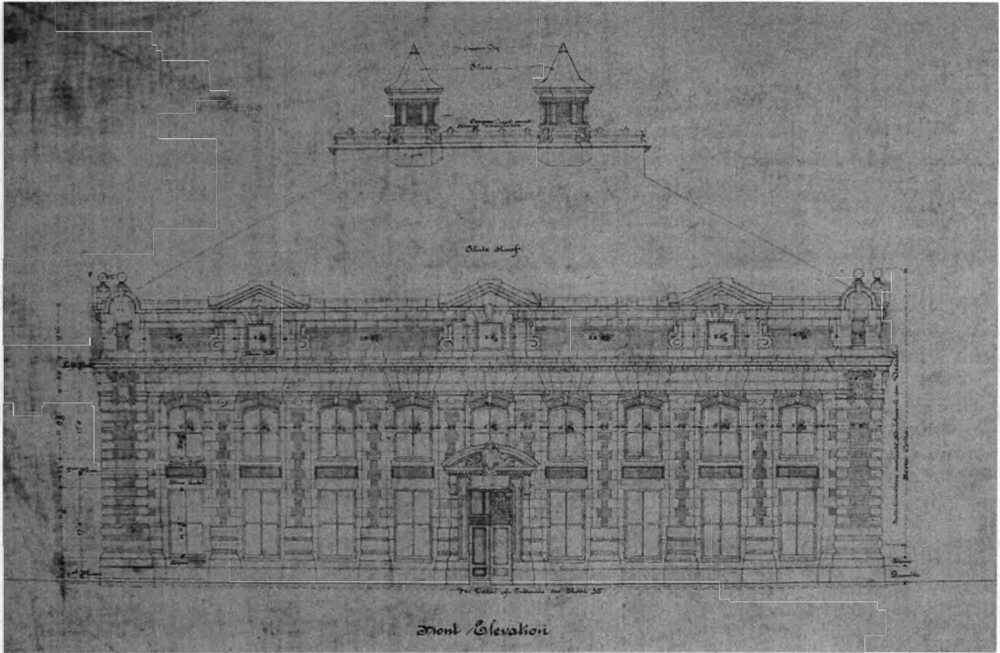
North Elevation Sewerage Pumping Station C.A. Didden & Son, Architects and Oscar Vogt, Associate Architect, ca. 1902 Department of General Services, Archives (Reeves Center, B-2)
