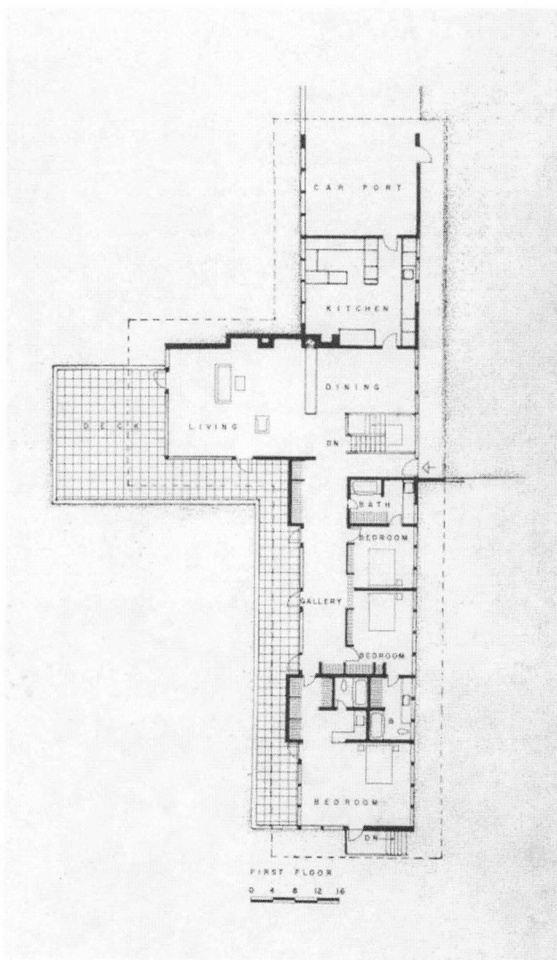
Willis Noll Residence first floor plan.
