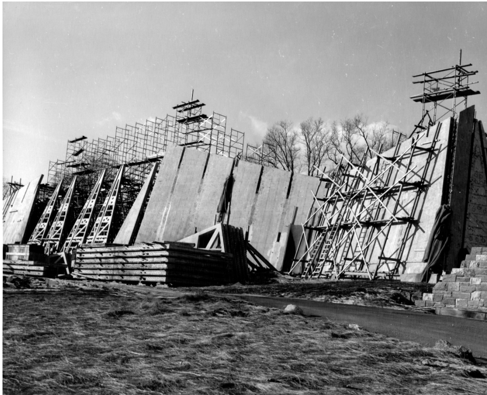
Figure 4: Sanctuary, south elevation, claustra panels under construction, camera facing NW Photograph DeLuca Construction, 1957 Courtesy DeLuca Construction, Stamford, Connecticut
