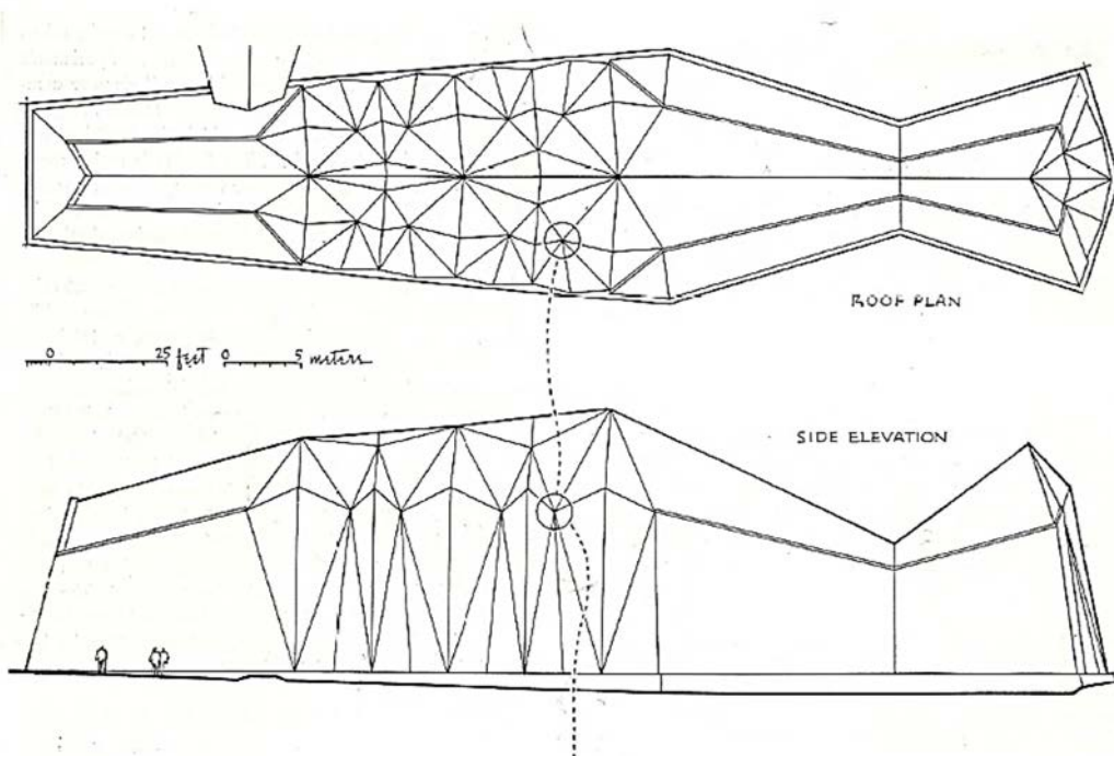
Figure 3: First Presbyterian Church Sanctuary, roof plan and side (south) elevation, sketch of final design without portal published in "P/A News Survey: Precast-concrete facets enclose piscine-form sanctuary," Progressive Architecture (April 1958): 107. Courtesy Wallace K. Harrison Papers, Avery Library, Columbia University
