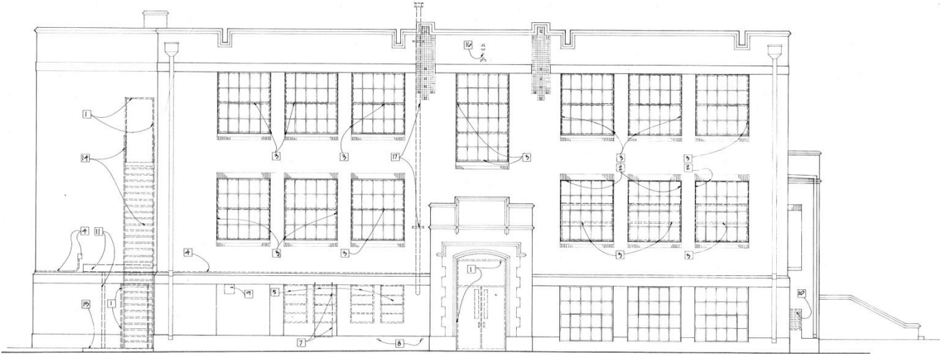
901 SOUTH ELEVATION
