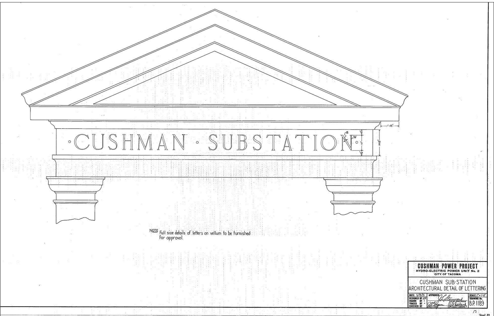
Figure 19. Design drawings of Cushman Substation, Architectural Detail of Lettering (over front entrance on south façade), December 1924. Image courtesy of Tacoma Power.
