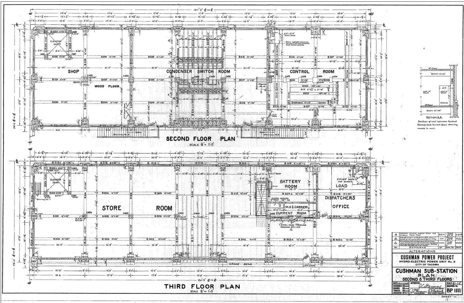
Figure 14. Design drawings of Cushman Substation, Plan of Second and Third Floors, December 1924. Image courtesy of Tacoma Power.
