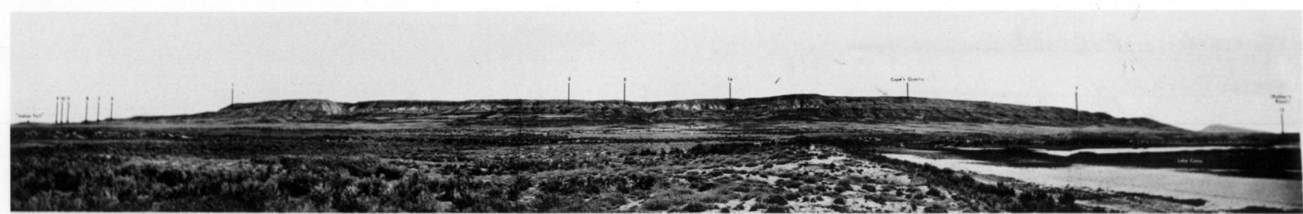
Fig. 12. Panoramic photograph of Green Hill taken from the shore of Lake Coeur just south of Coeur Station with the main section and localities shown.
