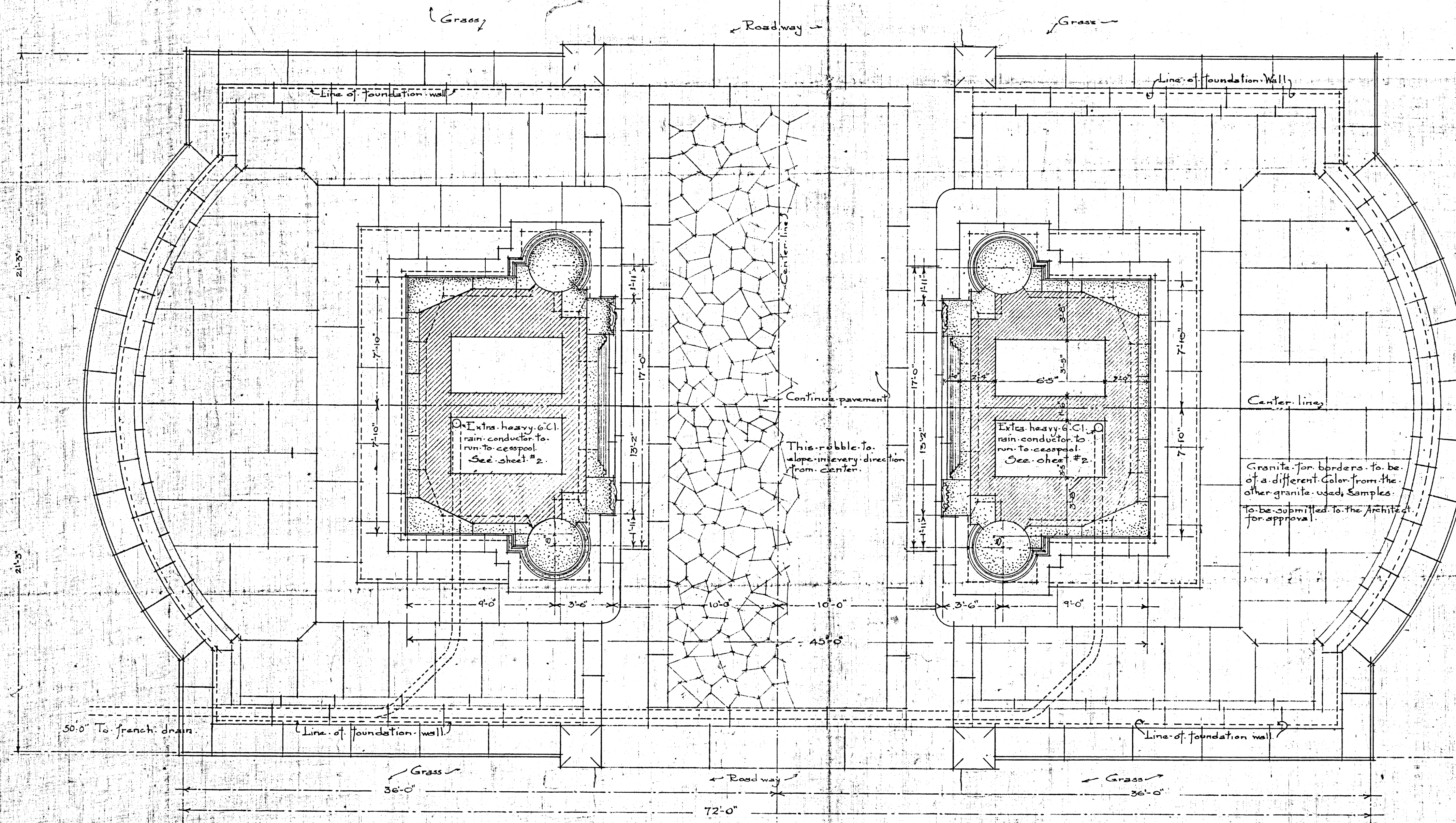
PLAN ABOVE BASE COURSE
