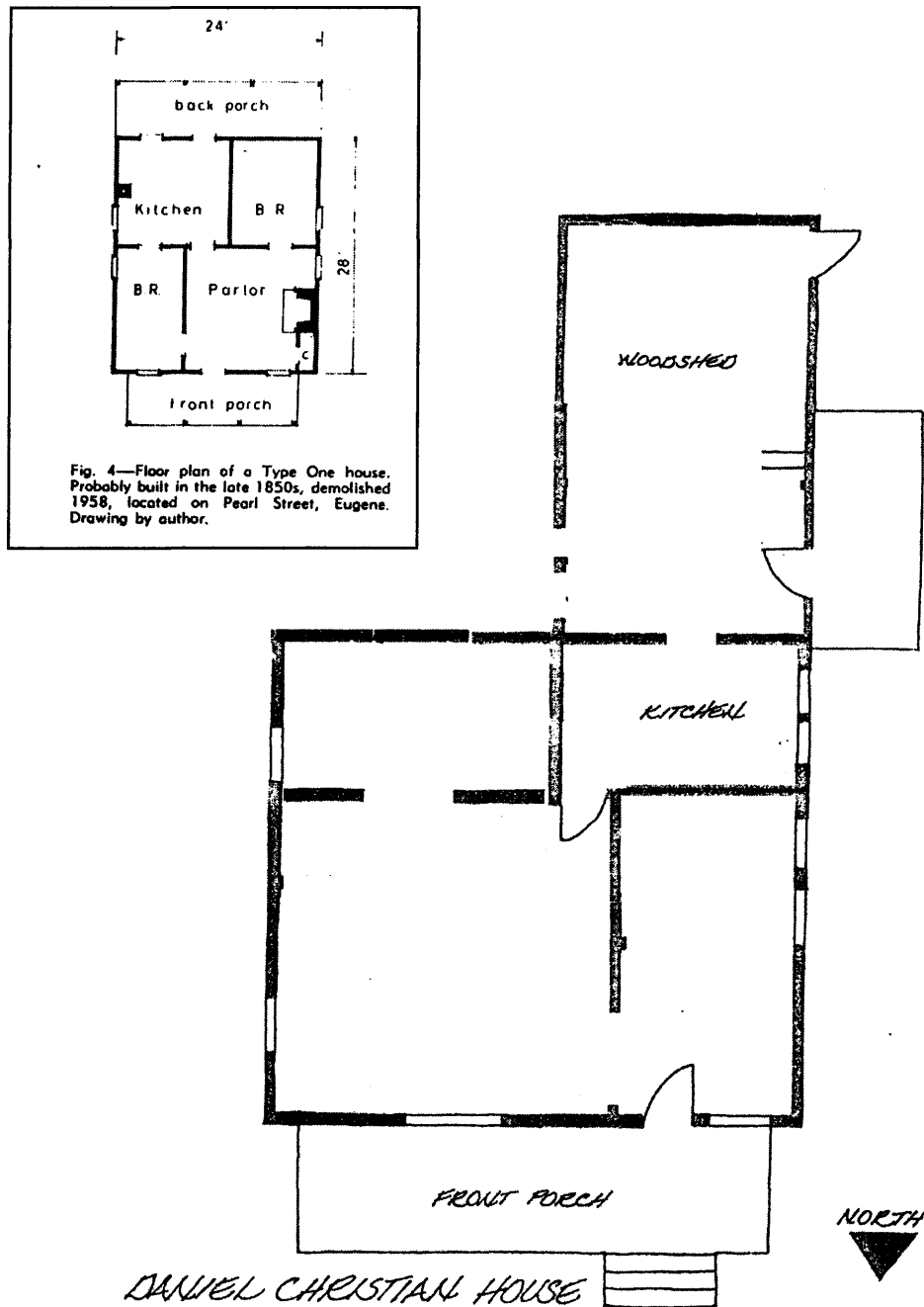
Figure. 18. Possible original configuration of first floor plan based on substructure arrangement and comparison to similar house described by Dole. Inset: Drawing from Dole's article "Farmhouse & Barn in Early Lane County" showing Type 1 house floor plan.
