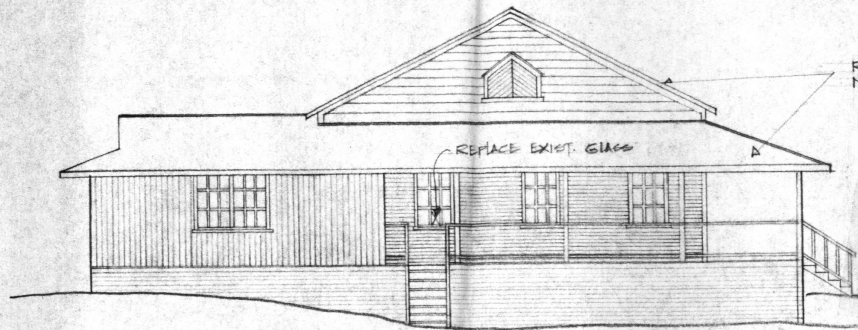
FRONT ELEVATION
