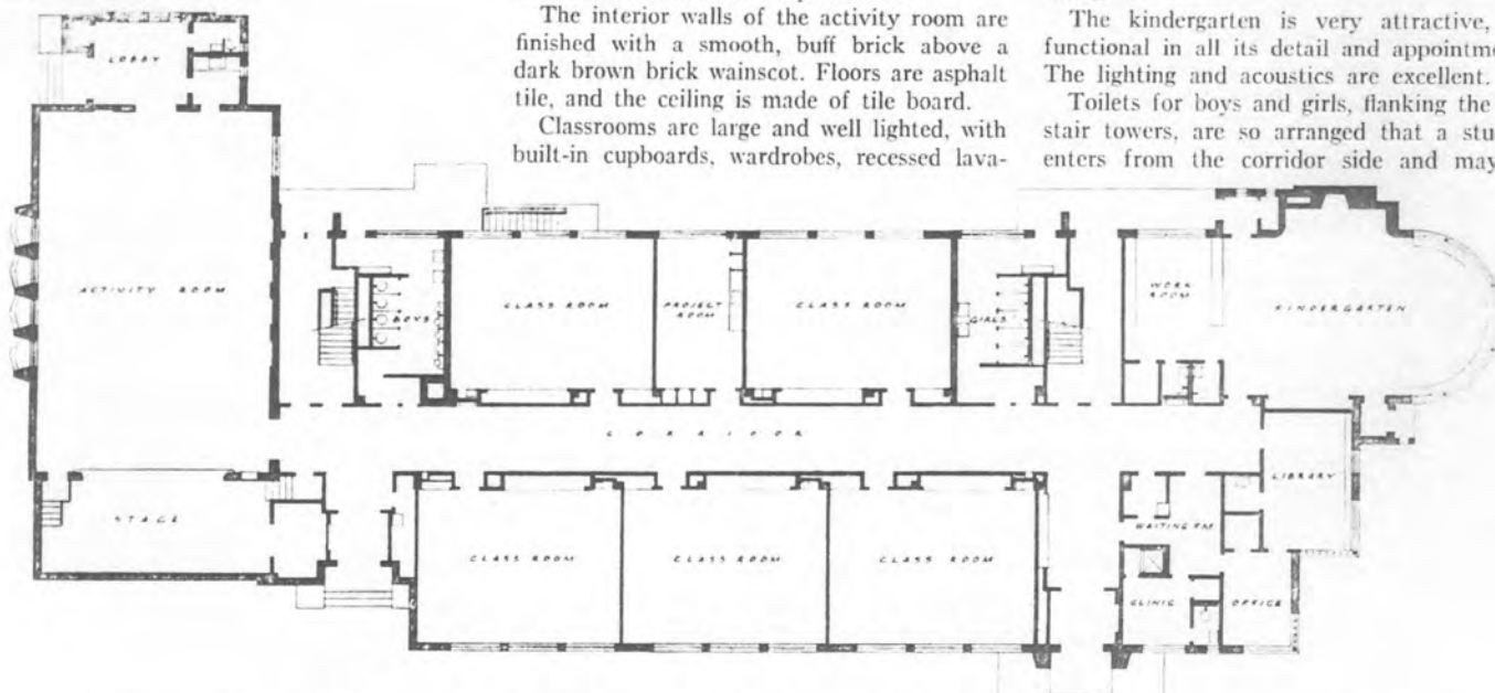
First Floor Plan, Garfield Elementary School, Abilene, Kansas. — Jos. W. Radotinsky, Architect, Kansas Cit, Kansas, and Frank Cayton, Associate Architect, Abilene, Kansas.
