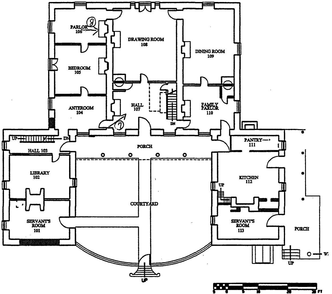
ADENA FIRST FLOOR 1/16" = 1'-0"
