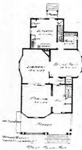
Figure 1: Design No. 81 from A few of the many Suburban and City Dwellings that have been erected by H. Galloway Ten Eyck, Architect (1895).
