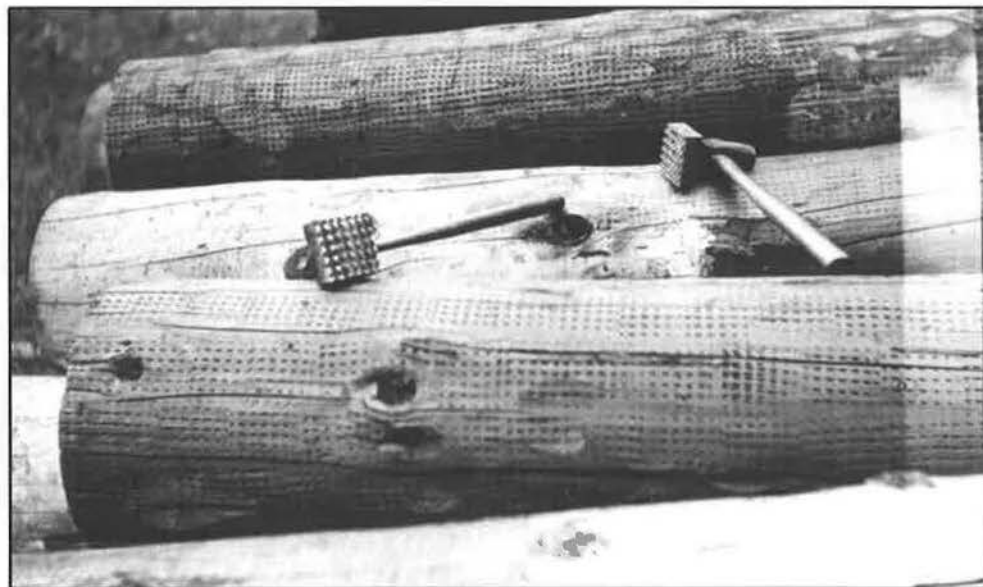
“Incised and treated guard rail posts and incising sledges. Sledges have 3/8" teeth on 3" square faces and weigh about six pounds.” Final Construction Report (1935-1936) on Red Lodge-Cooke City Approach Road to Yellowstone National Park, on Section D (Portion), Surfacing, Bituminous Base Treatment and Bituminous Road Mix. L. A. Deklotz, 1936. Photo No. 29309 from page 6.
