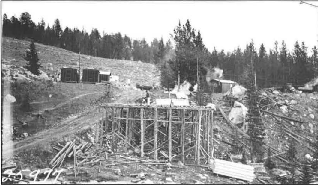
“Preparing for the construction of the Muddy Creek Bridge.” Final Construction Report (1931-1933) on Section B, Grading Red Lodge-Cooke City Approach Road to Yellowstone National Park, H. E. Mitchell, 1934. Photo No. 25977 from page 24.
