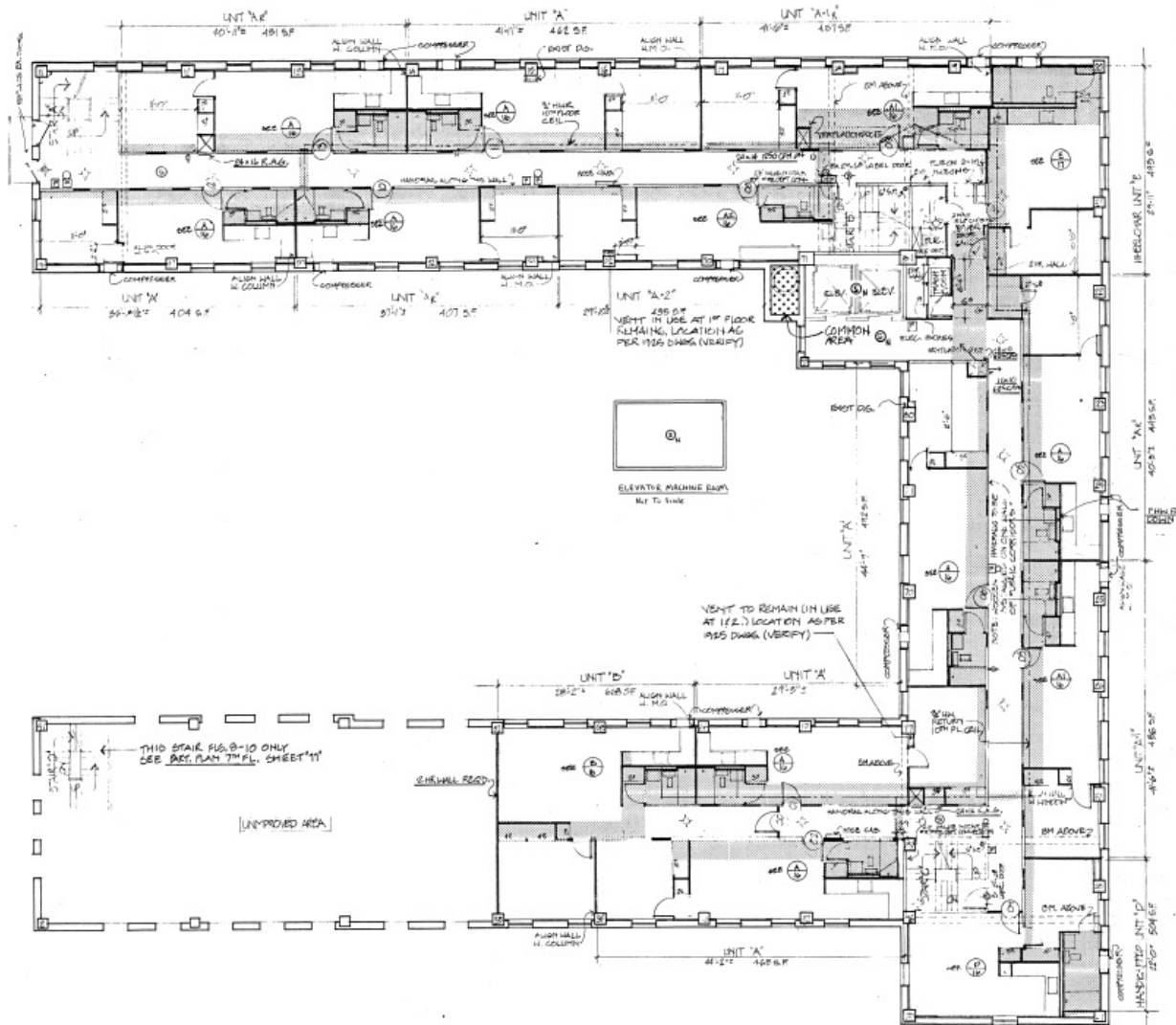
FLOOR PLAN 7-10
