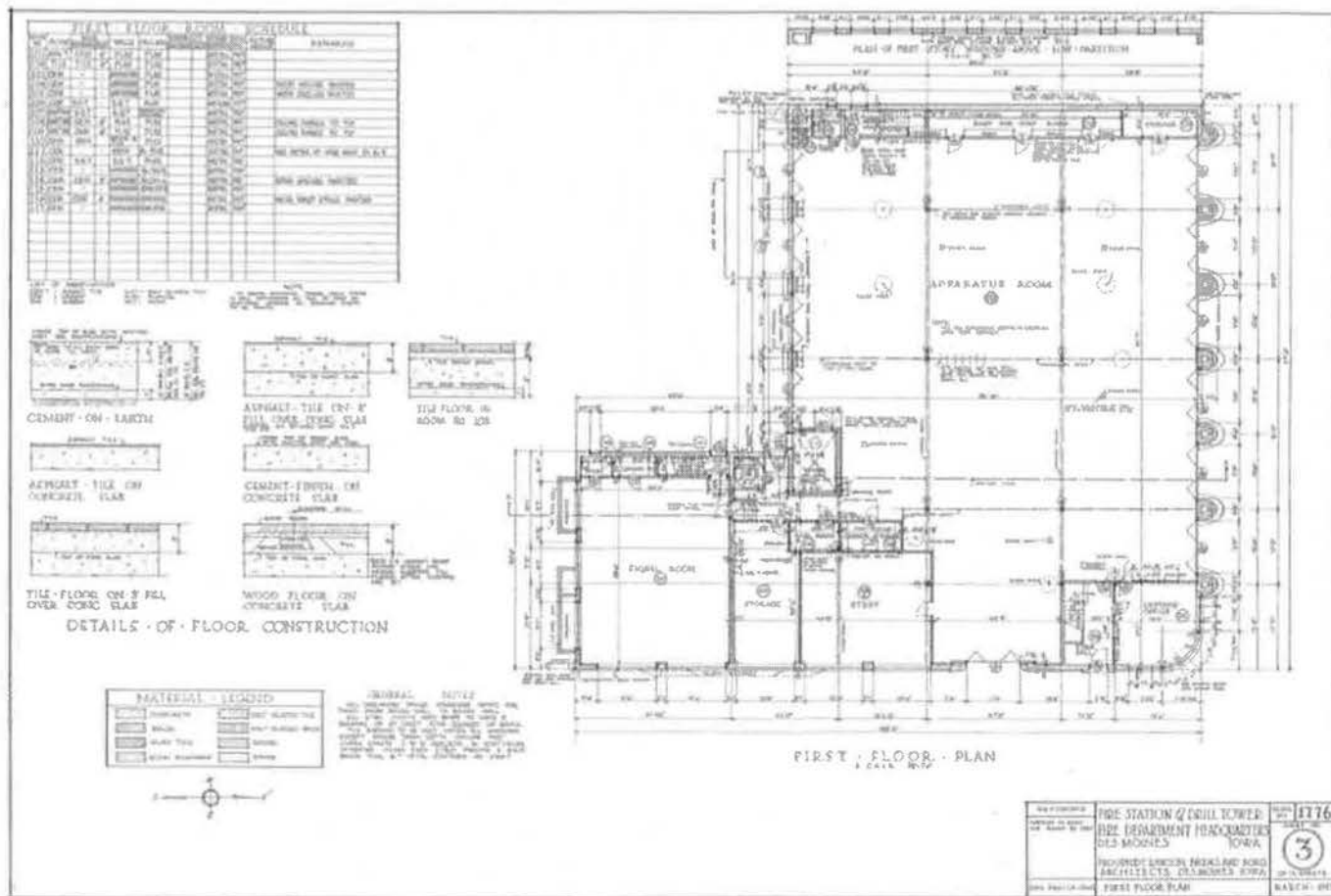
Figure 9. HISTORIC IMAGE – Fire station first-floor plan, March 1937
