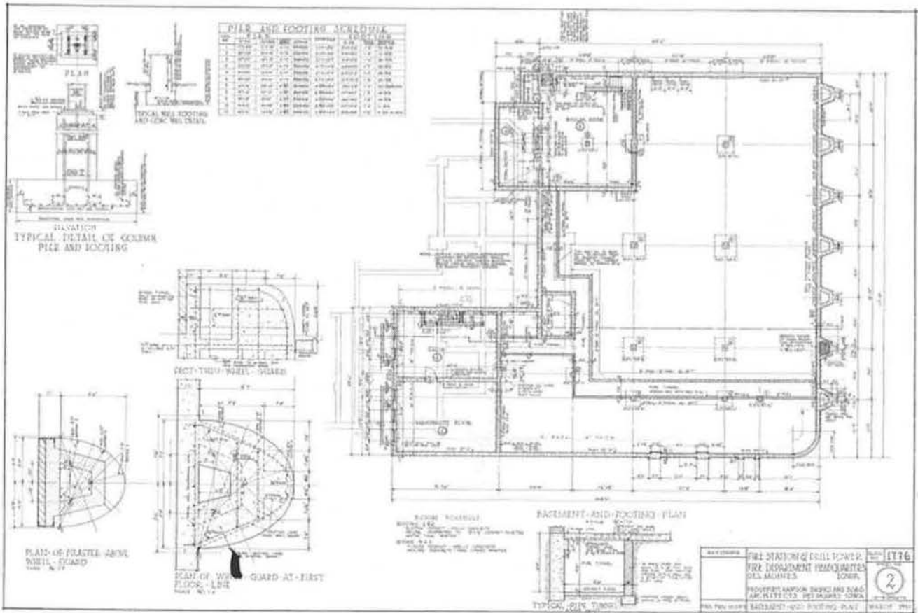
Figure 8. HISTORIC IMAGE – Fire station basement plan, March 1937
