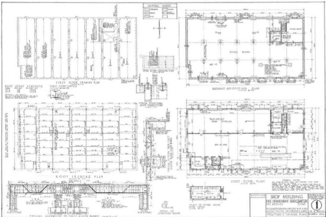
Figure 7. HISTORIC IMAGE – Shop Building floor plans, December 1936
