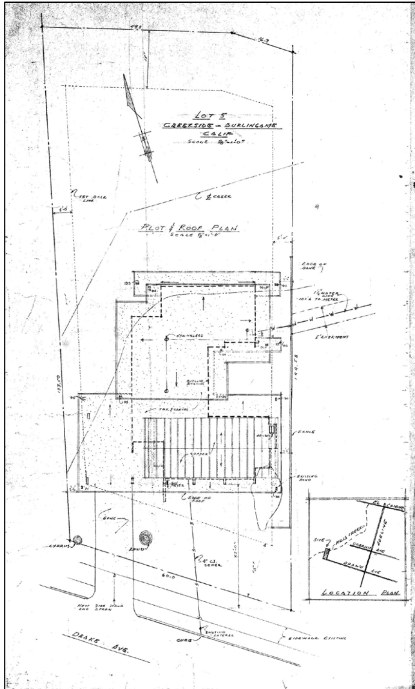
Figure P. From sheet 1 of original working drawings by Hannum & Whifler 1958. Plot and roof plan.
