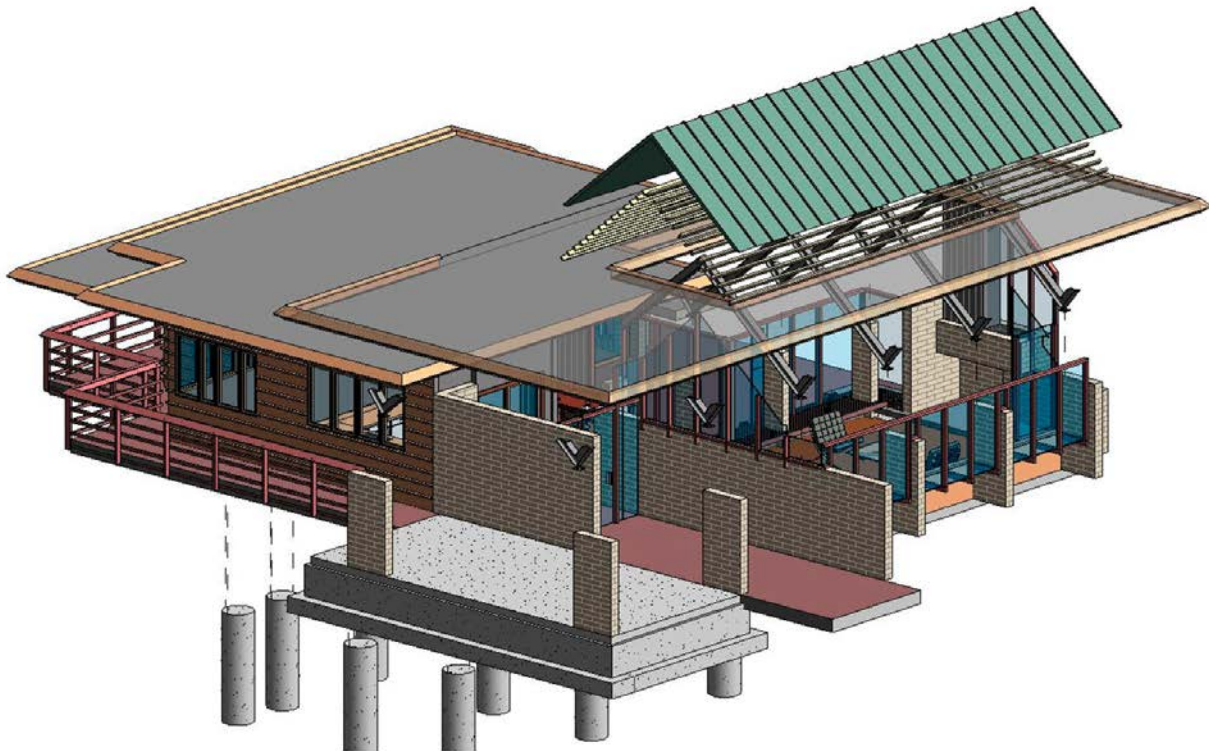
Figure M. Exploded front view showing concrete pier foundation, concrete masonry piers below W-shaped steel bents, glass curtain walls, and the 2x4 wood rafters supporting a copper clad roof. Revit model by Thomas Rex Hardy, AIA.
