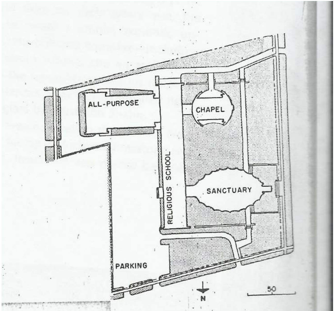
Temple Beth Zion Site Plan Source: Architectural Record, March 1968
