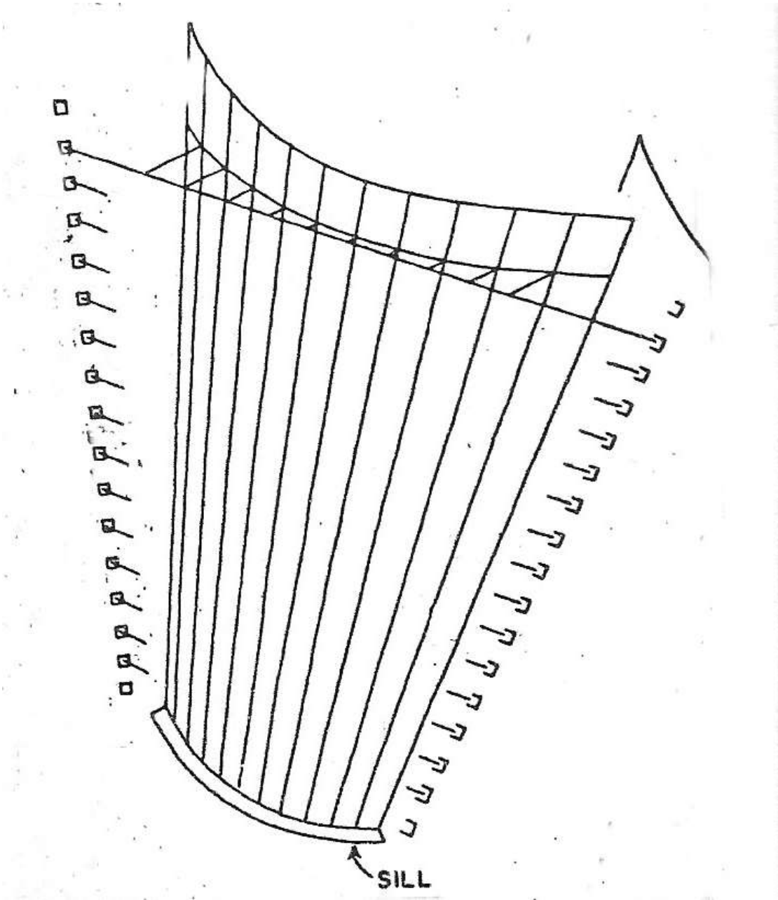
Lev Zetlin's stained glass window structure, balcony window Source: Architectural Record, March 1968.
