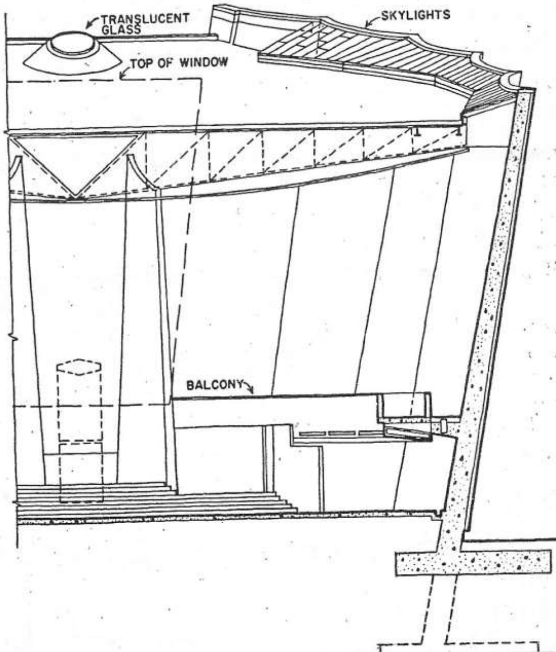
Cross-section of Sanctuary Source: Architectural Record, March 1968
