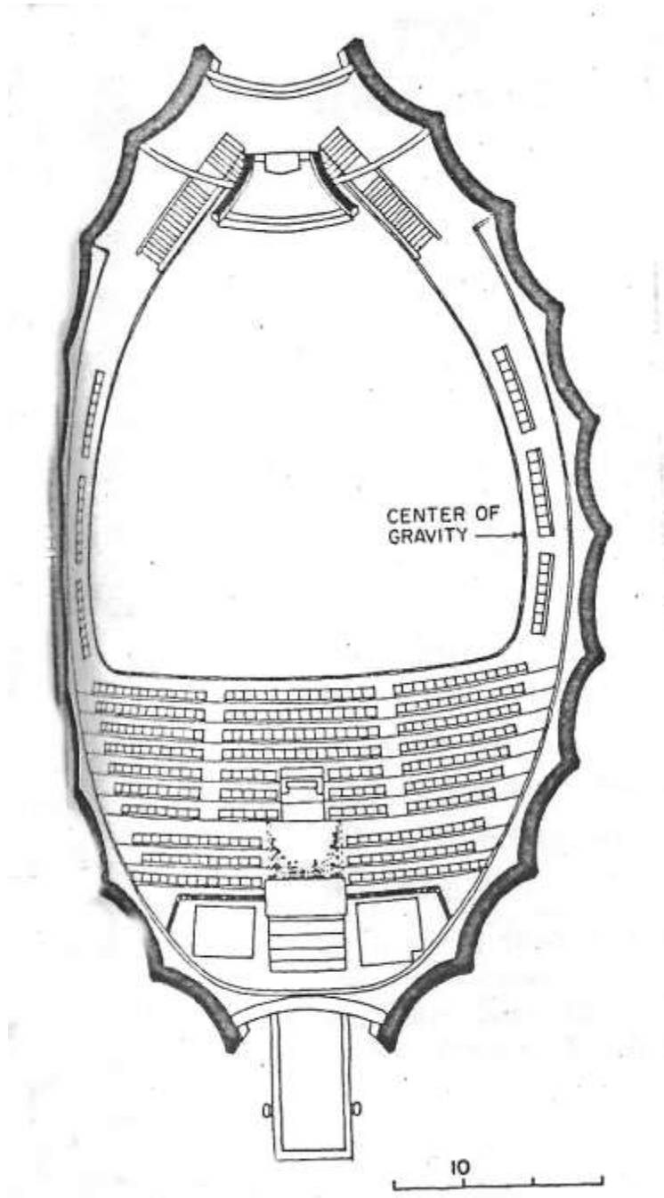
Plan of Sanctuary Source: Architectural Record, March 1968
