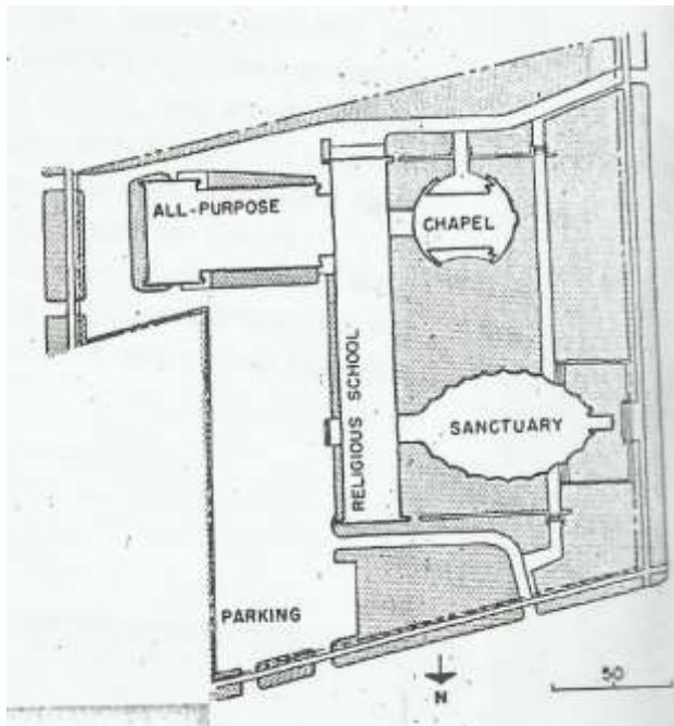
Temple Beth Zion Site Plan Source: Architectural Record, March 1968
