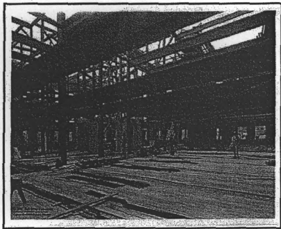
Figure 1, left: Construction Photograph, looking up from ground or first floor, showing the heavy steel structural framework and part of the concrete work in the background center. Courtesy of the Drawings and Documents Archive, Ball State University, 23-18B-007_s.t.
