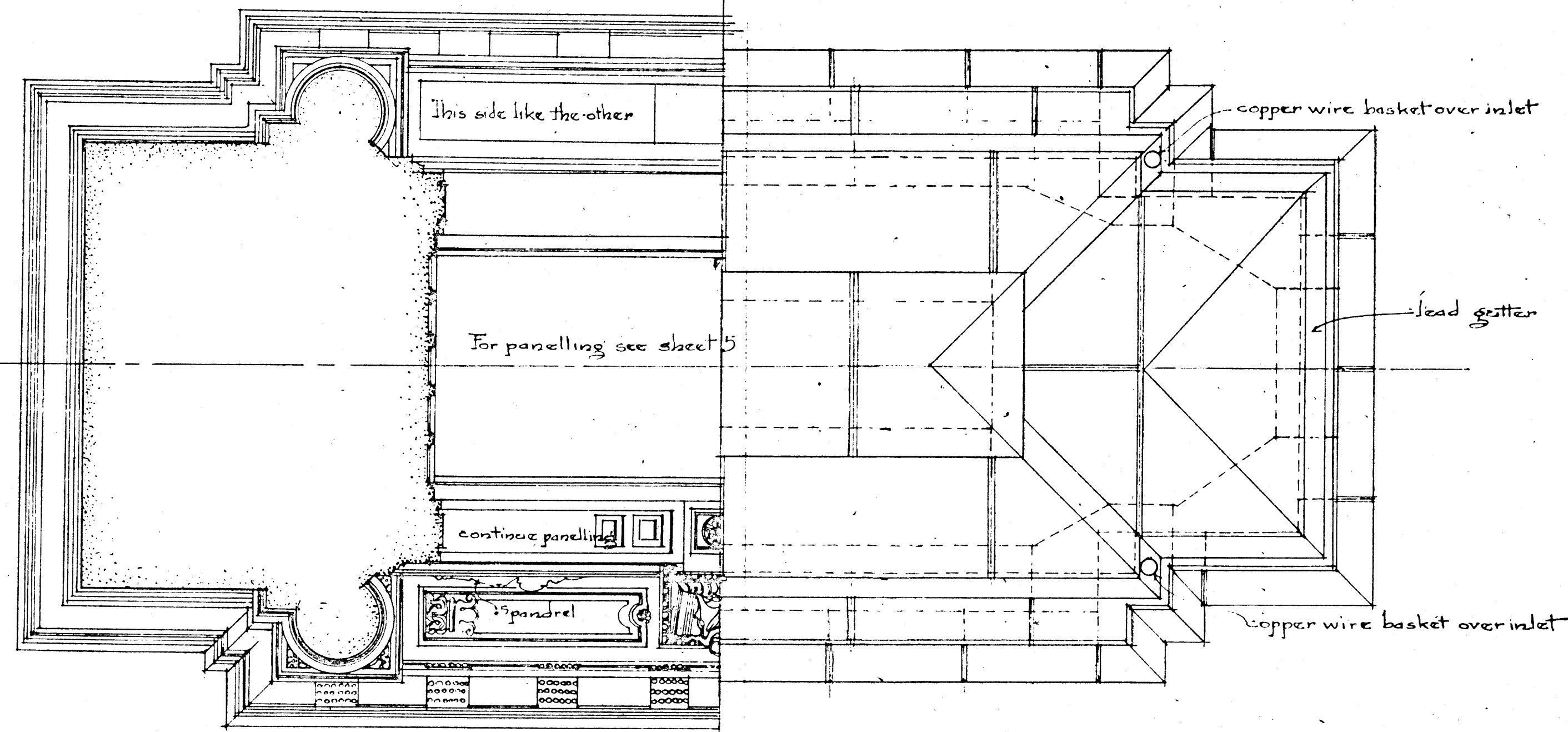
HALF PLAN AT LEVEL OF CENTER OF ARCH LOOKING VP
