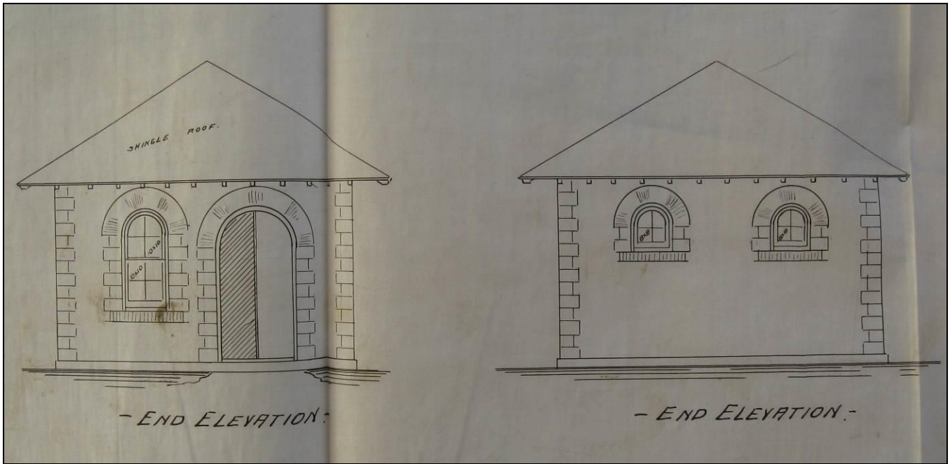
Figure 14. Tool House for Coeur d'Alene Park, City Eng'r's Office, May 1898 (no longer extant). Selected detail of elevations. Courtesy of City of Spokane Parks and Recreation Department.
