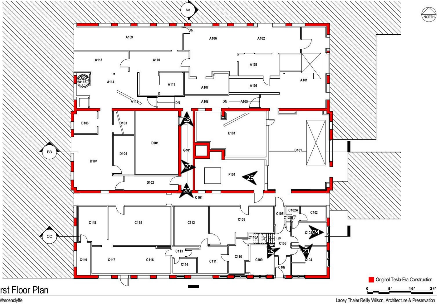
Figure 1. Wardenclyffe, First Floor plan and photo key.
