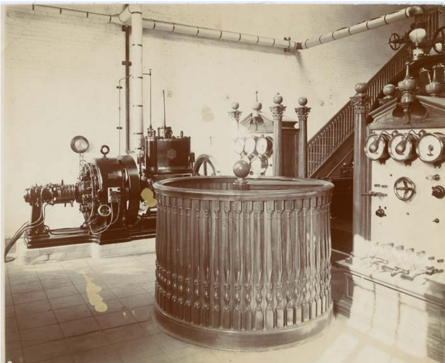
Figure 6. Interior of Wardenclyffe Laboratory Dynamo Room, looking north. Photograph courtesy of the Belgrade Museum.
