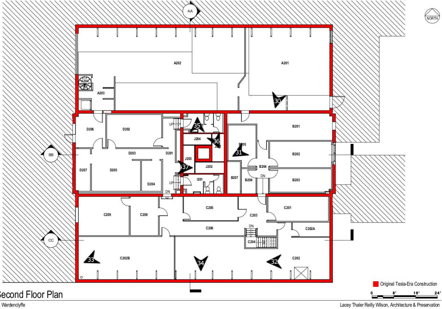
Figure 2. Wardenclyffe, Second Floor plan and photo key.
