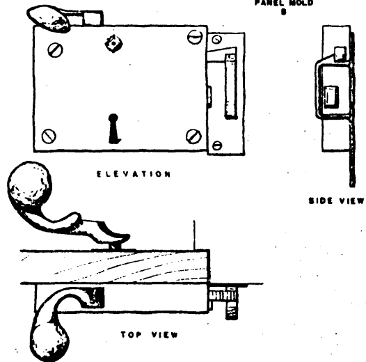
WROUGHT IRON BOX LOCK AND KEEPER SCALE 6"=1'-0"
