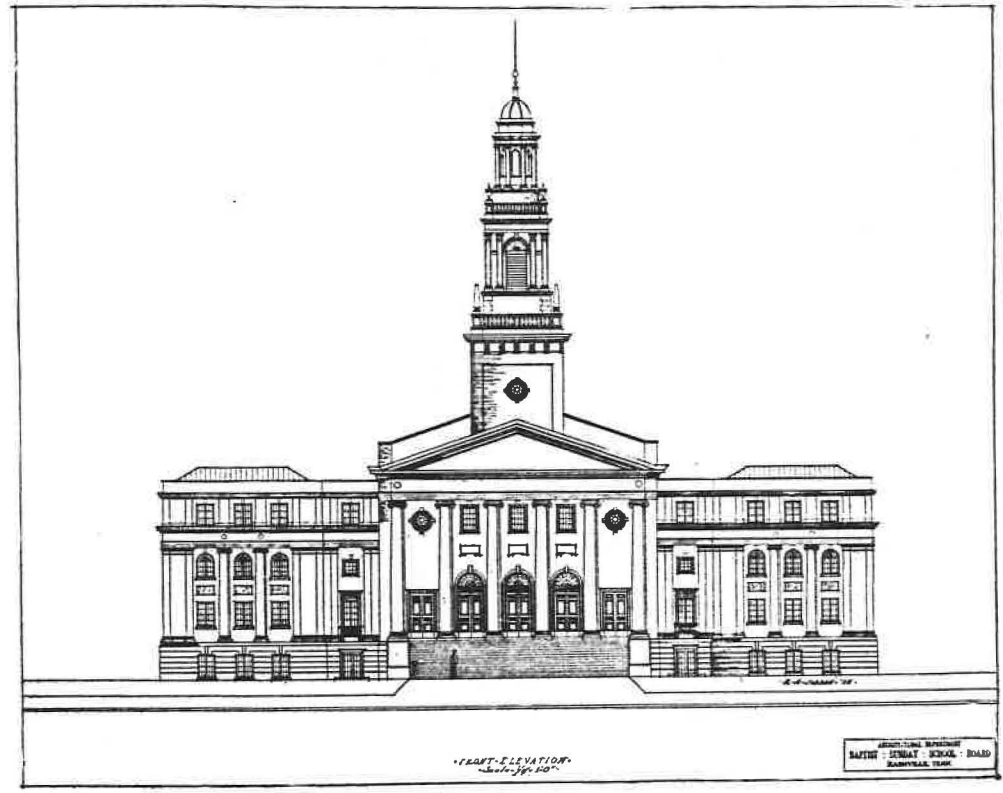
FRONT ELEVATION 1907 PRELIMINARY STUDY FOR THE CRESCENT HILL BAPTIST CHURCH, LOUISVILLE, KENTUCKY. Plan No. 1205 Designed by the Architectural Department, Baptist Sunday School Board
