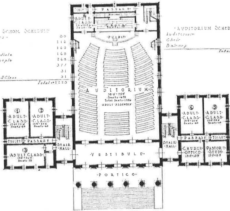
AUDITORIUM FLOOR PLAN Scale: 1/8" = 1'-0"
