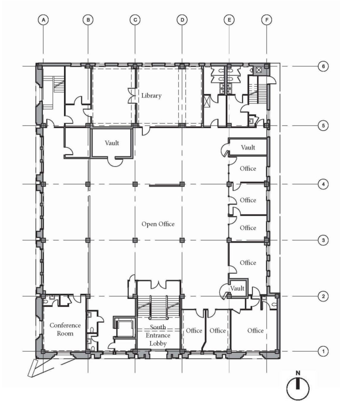
Figure 10. 1 st floor plan
