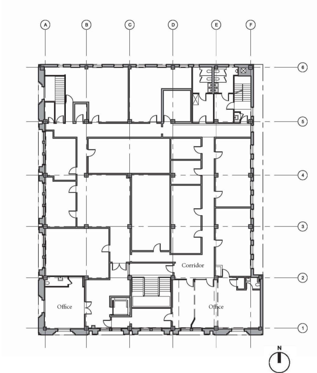
Figure 11. 2 nd floor plan
