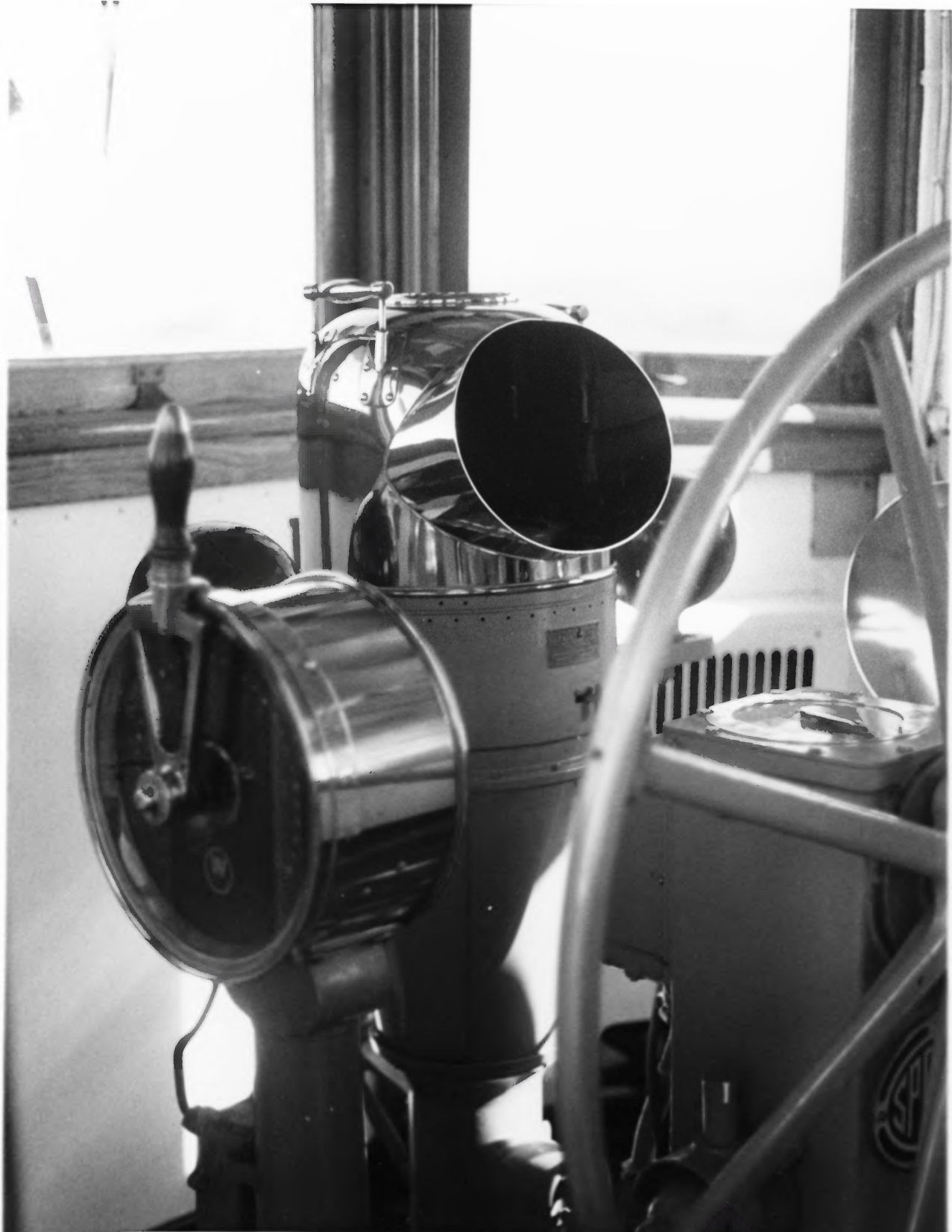
FIREBOAT CITY OF OAKLAND, EX-HOGA OAKLAND, CALIFORNIA Owner: UNITED STATES NAVY PILOTHOUSE INTERIOR, SHOWING ORIGINAL U.S.-NAVY ISSUED EQUIPMENT. Photo #9 by JAMES P. DELGADO, 1988 Courtesy of: NATIONAL PARK SERVICE
